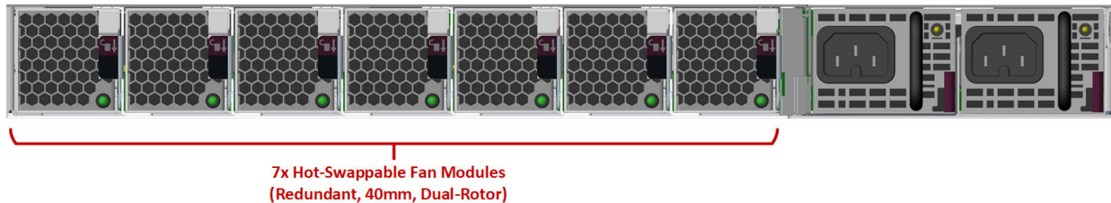
Figure 2. TPS TXE device - back panel
