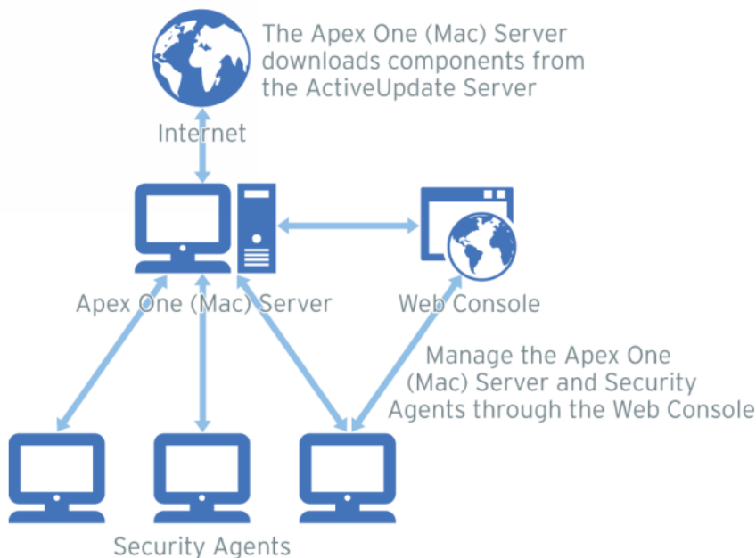
FIGURE 1-1. How the Trend Micro Apex One (Mac) server works
