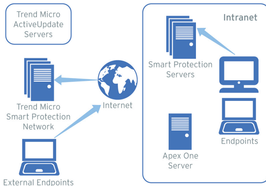
FIGURE 4-2. Query process
