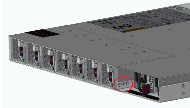
Figure 4. TippingPoint TPS 8600TXE devices - DC grounding screw holes to accept the lug connector attached to ground
